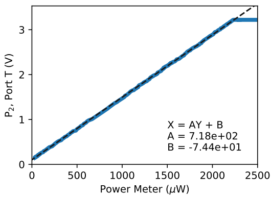
Figure 6: Typical power calibration for P_1 and P_2 .
