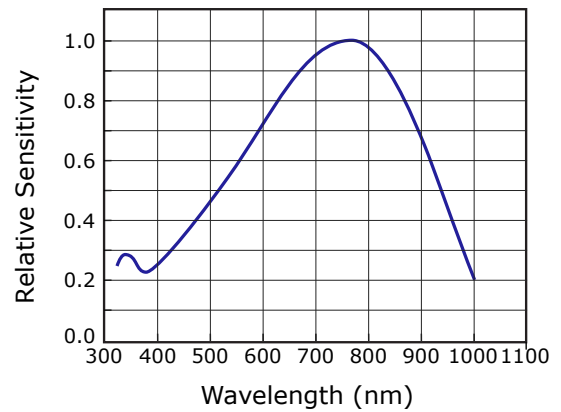
Figure 7: Spectral sensitivity
