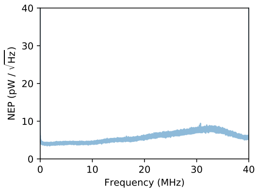
Figure 1: Digital noise floor at 1 kHz BW. 2
