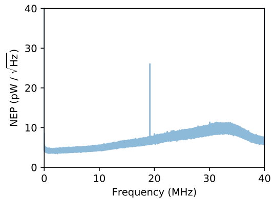
Figure 2: Digital noise floor at 10 Hz BW.
